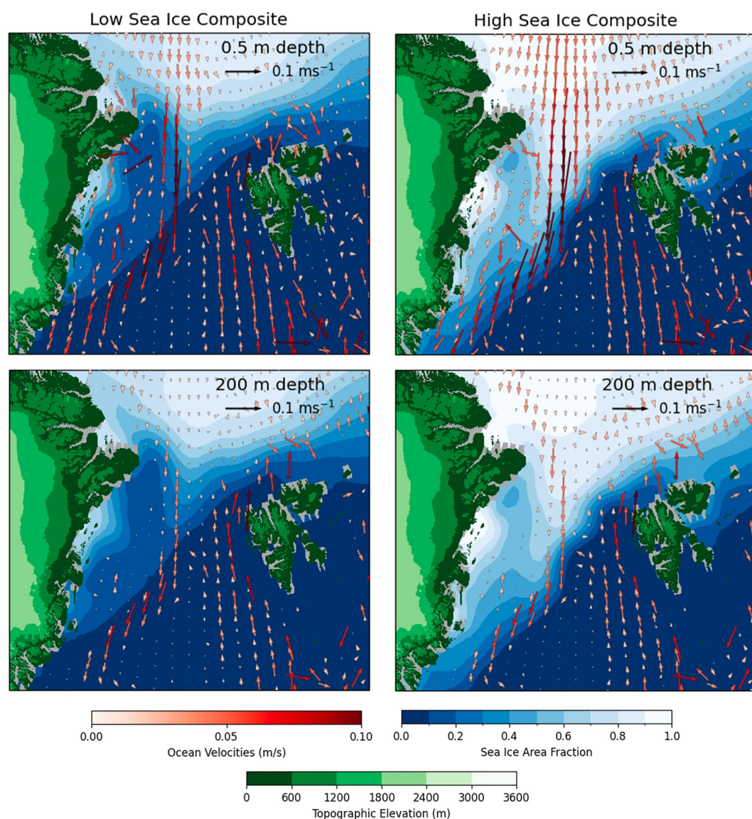
Figure 8. Composite mean August climatology using the 10 years with the highest and lowest sea-ice concentrations, respectively. The ERA5 sea-ice area fraction, the STRM30 topography and the ORAS5 ocean velocities at depths of approximately 0.5 m (upper row) and 200 m (lower row) are shown.
