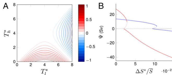
Fig. 1. Box model solutions for the magnitude of the overturning circulation \Psi ( \text{Sv} = 10^6 \text{ m}^3 \text{ s}^{-1} ) for the three salinity scenarios. (A) Freshwater case with surface temperature forcing T_h^* and T_l^* (°C), of the high and low latitude box, respectively, in the range 0–8 °C, contour interval 0.1 Sv. Positive circulation occurs when T_h^* < T_l^* < 8 - T_h^* (assuming T_h^* < T_l^* ). (B) Mid- (blue) and high (red) range salinity scenarios, dotted lines indicate unstable solutions, \Delta S^* is the gradient in salinity forcing, and \bar{S} is the mean salinity. The scaling \Delta S^* \propto \bar{S} means direct comparison is possible when \Delta S^*/\bar{S} is varied. The range presented is equivalent to 0–5 and 0–38 g·kg -1 for \Delta S^* in the mid-range and high range salinity cases, respectively. A salinity-driven circulation occurs when \Delta S^*/\bar{S} > 0.105 and 0.03, respectively.
