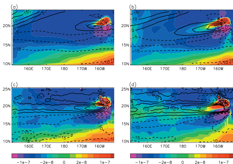
Figure 3: Wind stress curl (colour, Nm^2/m ) and ocean zonal current at 35m (contours at 5cm s^{-1} intervals, eastward currents solid, westward currents dashed). (a) lowest resolution (HadGEM), (b) higher resolution atmosphere, (c) higher resolution ocean, and (d) high resolution atmosphere and ocean (HiGEM).
