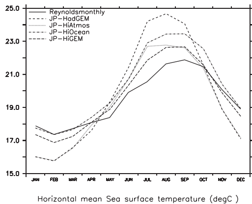
Horizontal mean Sea surface temperature (degC)
