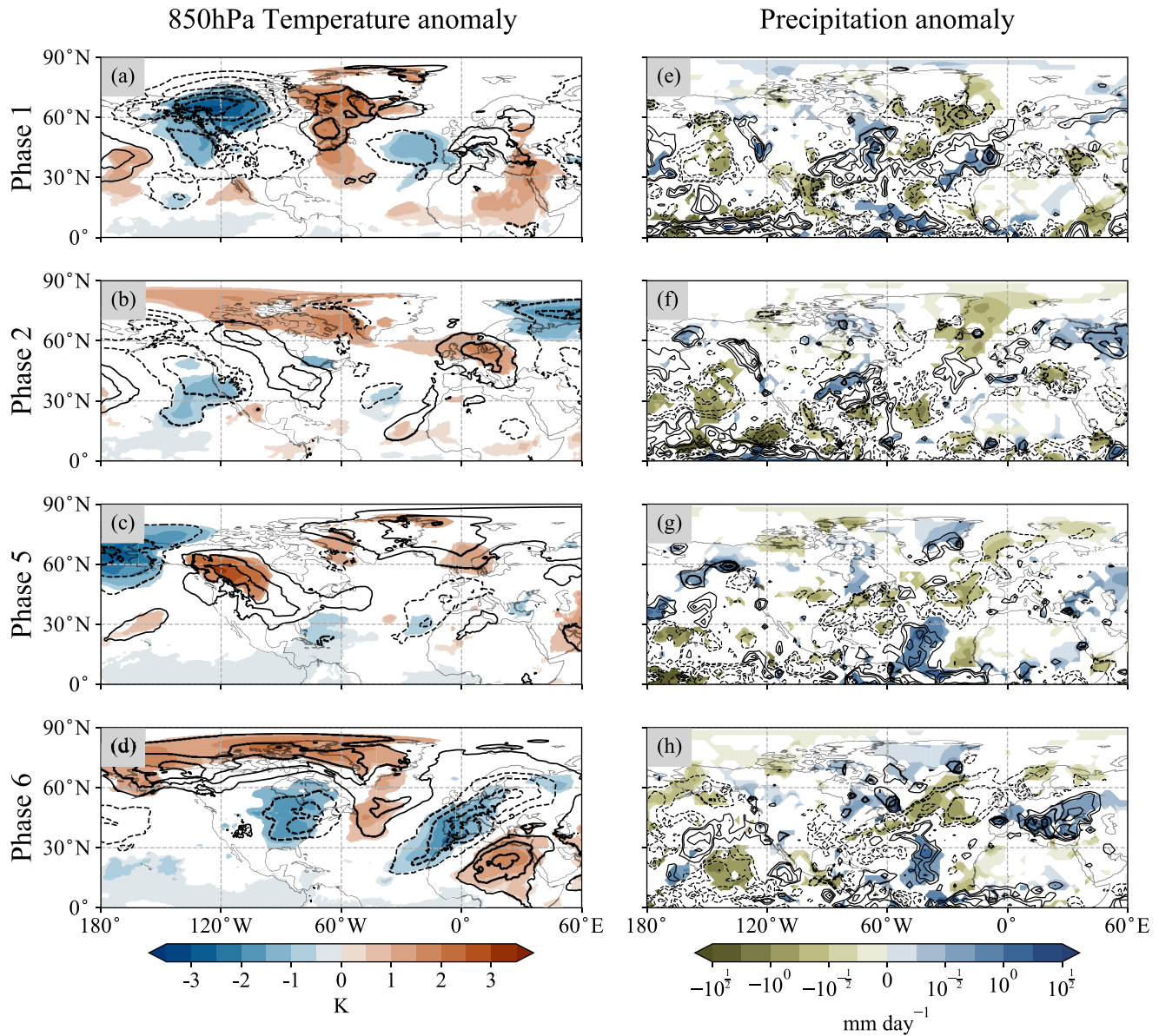
Figure 4. Change in 10-day lagged composites of (a–d) 850-hPa temperature and (e–h) precipitation anomalies over North America, Europe, and North Africa for MJO phases 1, 2, 5, and 6 (see Figure S4 in Supporting Information S1 for remaining phases). Difference—period two (1997/98–2017/18) minus period one (1974/75–1996/97)—is color shaded wherever it is significant at the 95% level, with change in precipitation anomaly plotted on a logarithmic scale. Period two composites are overlaid as black contours for reference. Solid contours represent positive values, dashed contours represent negative values and the zero contour has been omitted. Contour levels are the same for the line contours as they are for the shaded contours.
