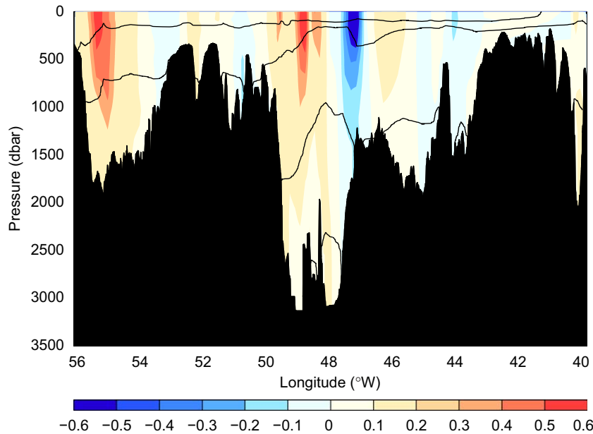
Fig. 12. Geostrophic velocity in \text{m s}^{-1} referenced to LADCP/ADCP profiles for station pairs along the North Scotia Ridge. Dark lines denote water mass boundaries in neutral density, with values as defined in Fig. 5.
