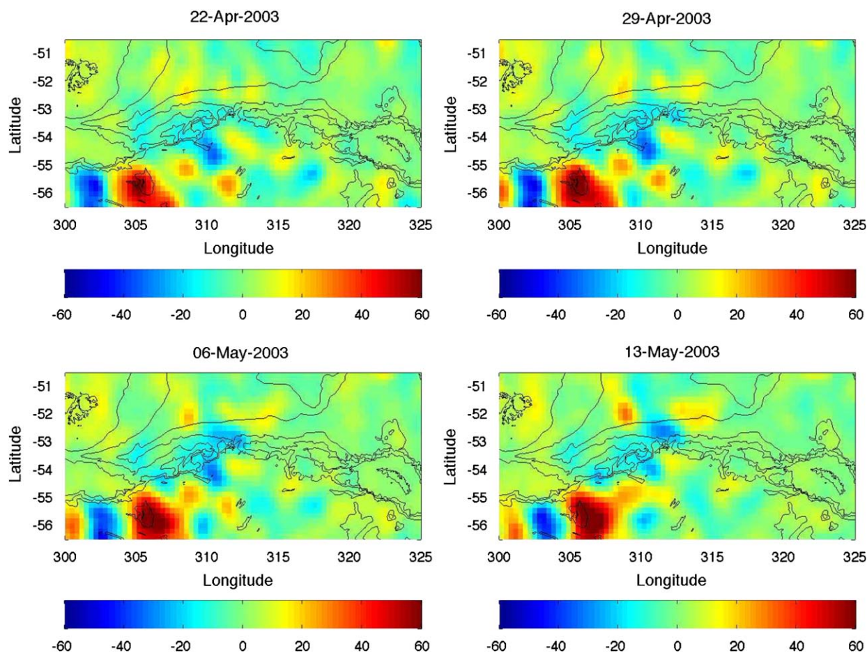
Fig. 16. Sequence of sea surface height (SSH) anomalies spanning the time period of the cruise, specifically 22 April–13 May 2003. Units are in cm. Note in particular the negative SSH anomaly in the vicinity of Shag Rocks Passage during May 6–13, indicative of a cold-core (cyclonic) eddy present here at this time.
