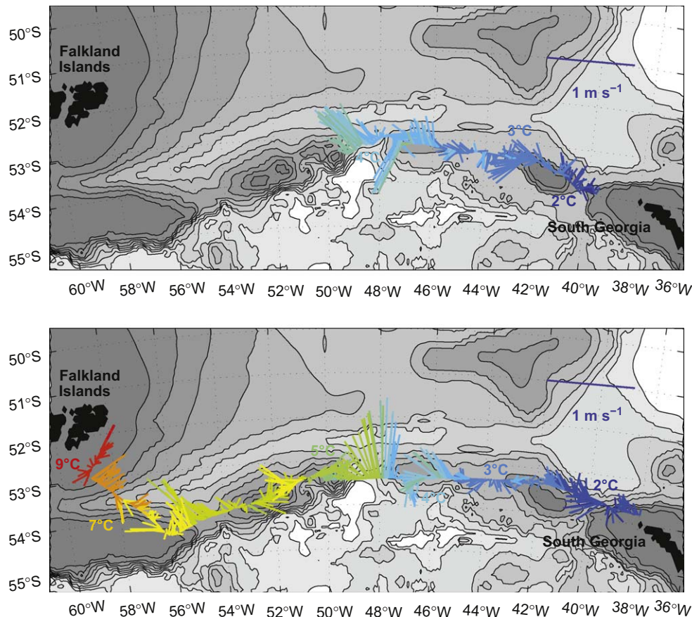
Fig. 2. Underway ADCP velocity vectors, averaged over 54–102 m, with 10 min time bins smoothed with an hourly running mean. Velocity vectors are coloured by surface water temperature, which is between 2 and 9 °C, in 0.5 °C intervals. The thermosalinograph measured water temperatures from an intake at approximately 5 m depth. Velocity values are indicated by the length of the lines, with a standard 1 \text{ m s}^{-1} line shown at the top right of the figure. The lower figure shows the outward track along the North Scotia Ridge, while the upper figure shows the corresponding return track along the ridge to Shag Rocks Passage. Once Shag Rocks Passage was crossed on the return leg of the cruise, the ship took a direct route to the Falkland Islands rather than following the ridge. For this reason, only data for half of the return leg is presented here.
