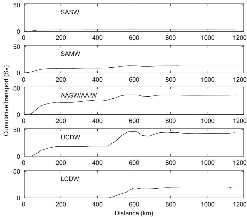
Fig. 14. Cumulative volume transports, accumulated from west to east, for water masses SASW, SAMW, AAIW/AASW, UCDW, and LCDW for the North Scotia Ridge.
