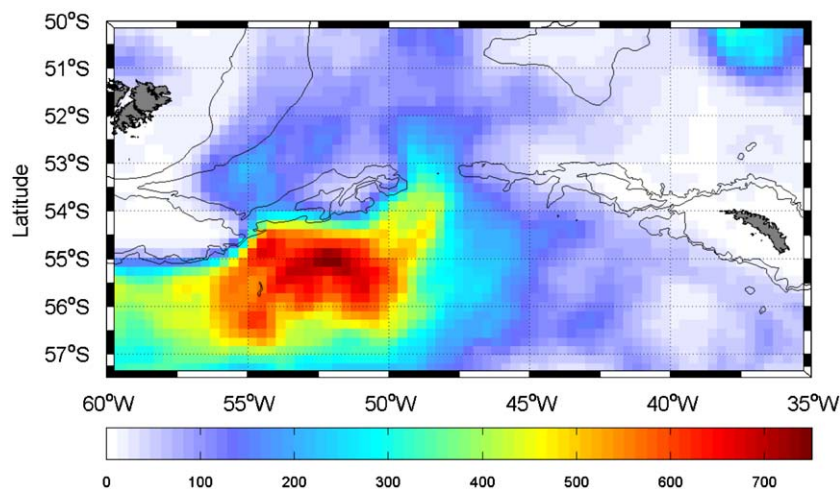
Fig. 15. Eddy kinetic energy (EKE) calculated from the AVISO joint TOPEX/ERS sea level anomaly product, covering the period 1992–2005. Units are in \text{cm}^2 \text{s}^{-2} .
