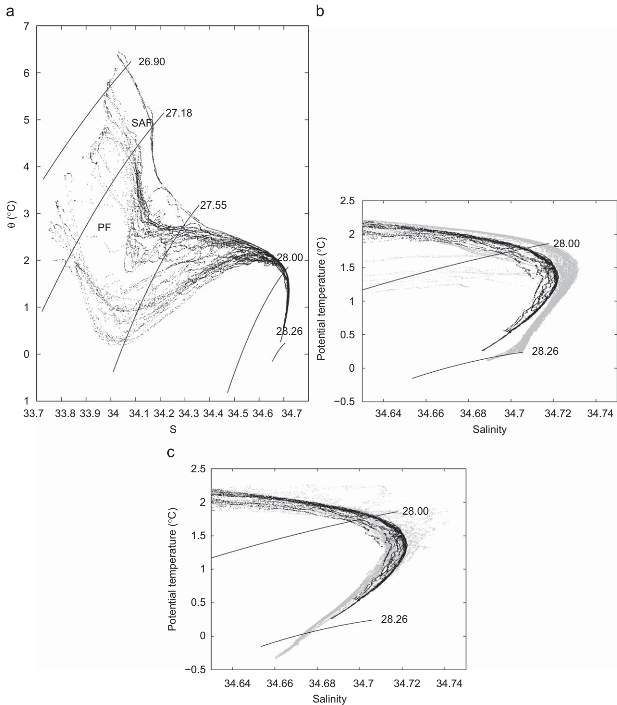
Fig. 9. (a) Potential temperature versus salinity, for the 49 CTD stations occupied along the North Scotia Ridge (black dots). Voids in \theta - S space mark the SAF and PF. Lines of neutral density (black lines, water mass separations) (Jackett and McDougall, 1997) are as for Fig. 5. (b) Close-up of densest water classes for the North Scotia Ridge (black dots) and for Drake Passage (grey dots—ALBATROSS cruise data from Naveira Garabato et al., 2002; stations for the ALBATROSS cruise are shown in Fig. 1). (c) Close-up of the densest water classes for the North Scotia Ridge (black dots) and for the Falkland Plateau/Georgia Basin (grey dots—ALBATROSS cruise data from Naveira Garabato et al., 2002; stations for the ALBATROSS cruise are shown in Fig. 1).
