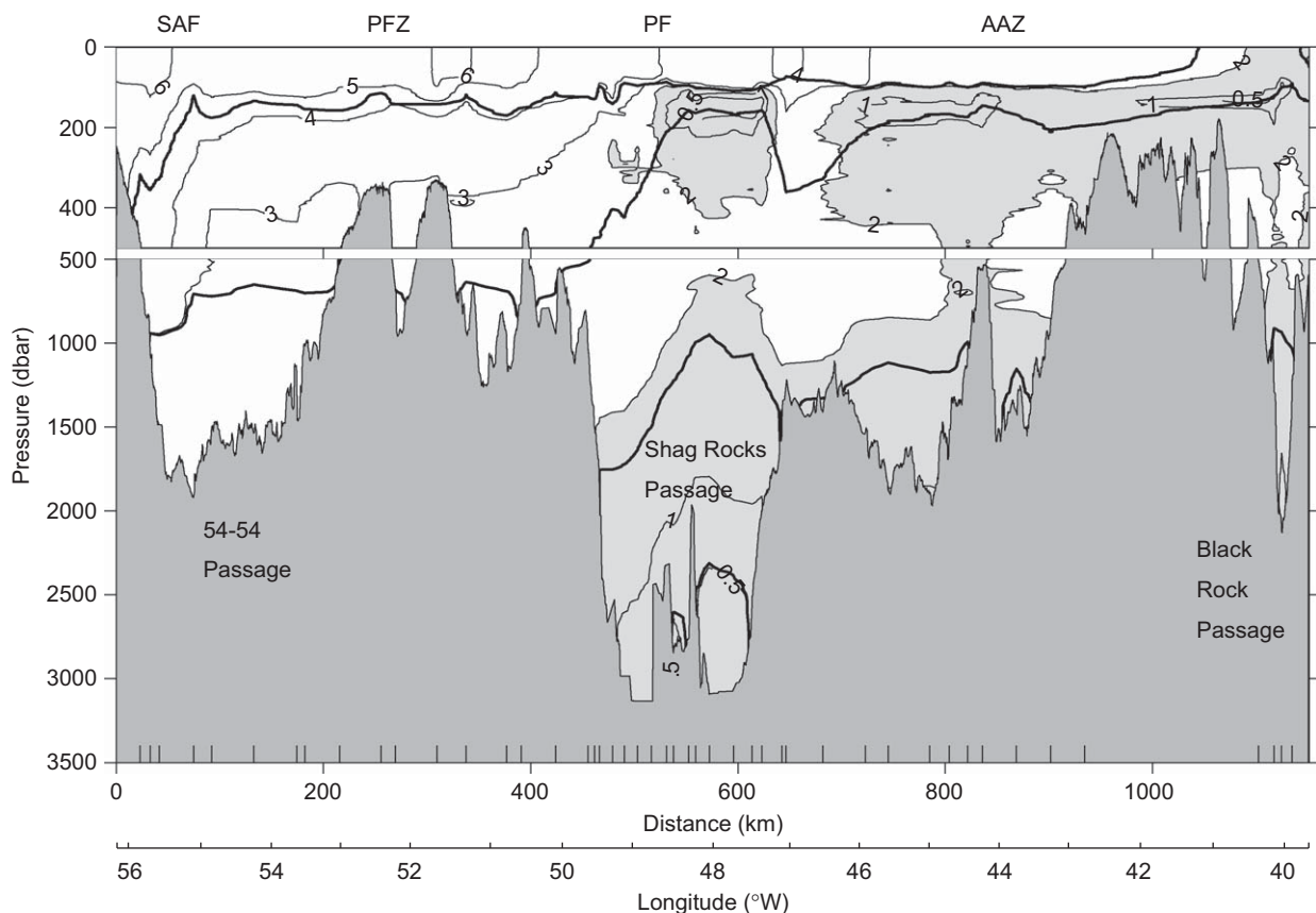
Fig. 3. Potential temperature section for the North Scotia Ridge. Values colder than 2 °C are shaded grey. Dark lines denote water mass boundaries in neutral density, with values as defined in Fig. 5. The location of the Polar Front (PF) and Subantarctic Front (SAF) are marked, with the Polar Frontal Zone (PFZ) and Antarctic Zone (AAZ) indicated. Station locations are shown along the lower axis.
