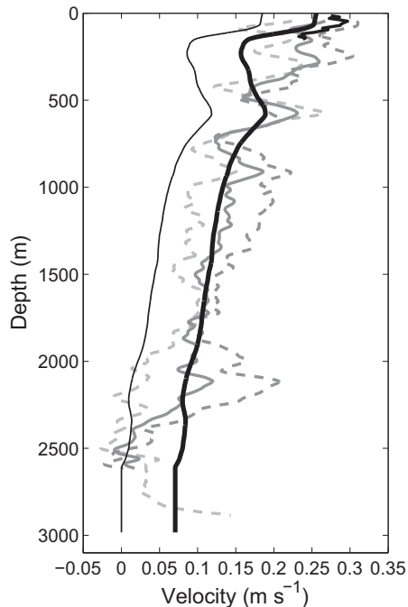
Fig. 10. Geostrophic shear for the pair of stations located at 49.1°W and 48.9°W, in Shag Rocks Passage. The thin black line is the geostrophic profile derived from CTD data, before any adjustments. The thick black line is the geostrophic profile adjusted by a constant offset based on the average value of the LADCP data. The 150 kHz LADCP data are shown as grey broken lines. The darkest grey line is the mean of the corresponding light grey dashed (eastern station) and medium grey dashed (western station) lines. The short black solid line is the ship-mounted ADCP data to 150 m depth.
