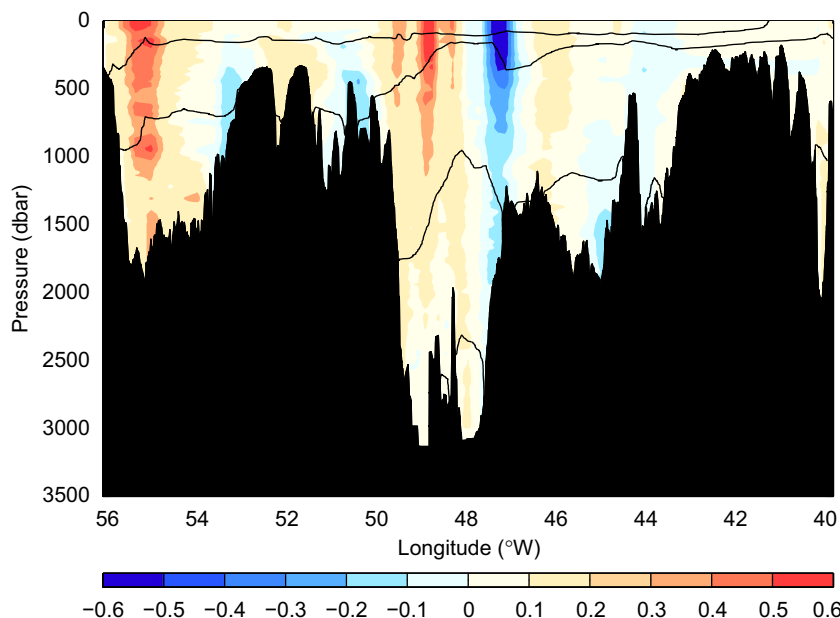
Fig. 11. LADCP velocity in \text{m s}^{-1} for station pairs along the North Scotia Ridge. Dark lines denote water mass boundaries in neutral density, with values as defined in Fig. 5.
